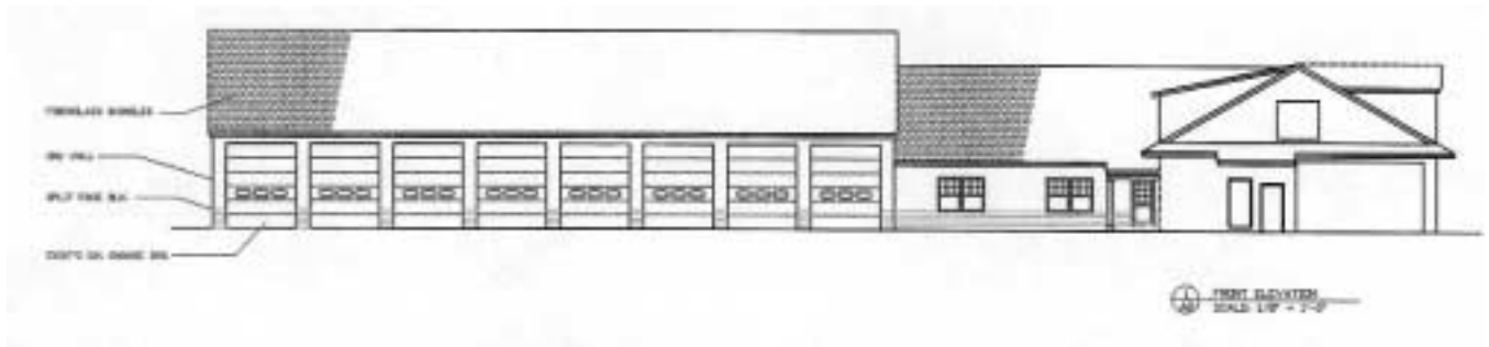
Front Elevation
